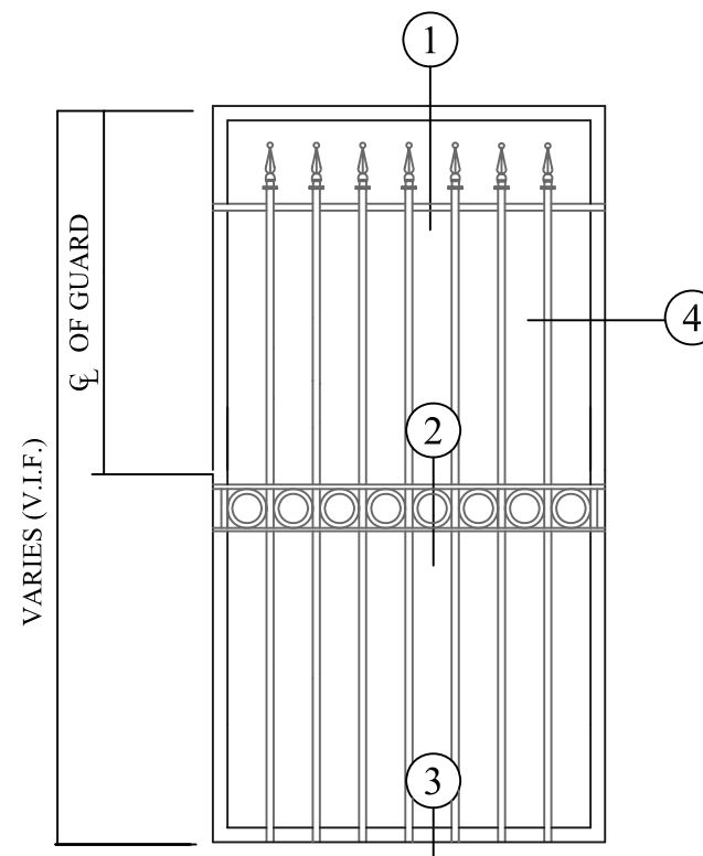
STEEL ARCHITECTURAL BAR GUARD ELEVATION
